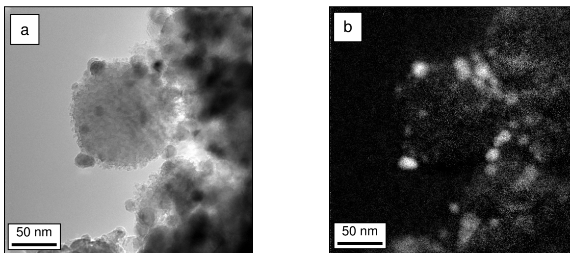
Figure 2. Nickel steam-reforming catalyst on MgAl_2O_4 support, a) TEM bright field image, b) Ni map of the same location, energy filtered TEM image, three-window method, Ni L_{23} edge.
